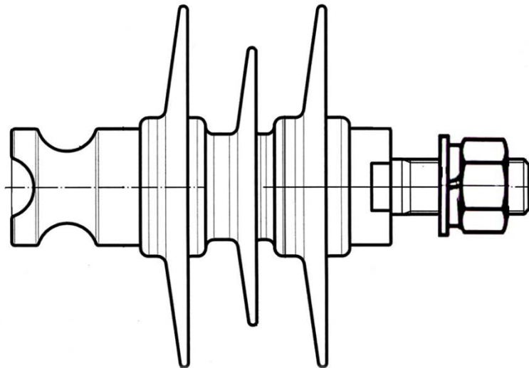
Fig. 11KV 10KN Composite Pin Insulator
