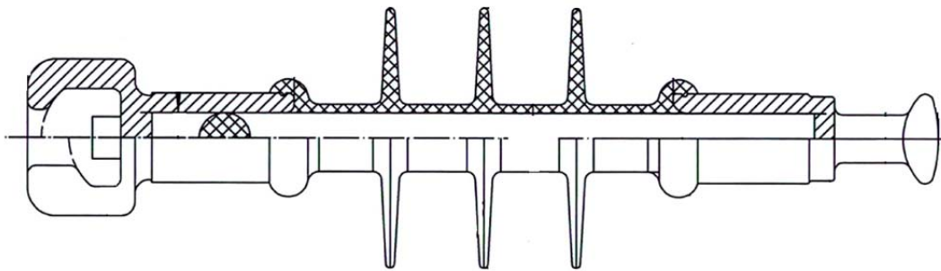
Fig. 11KV 70KN Composite Suspension Insulator
