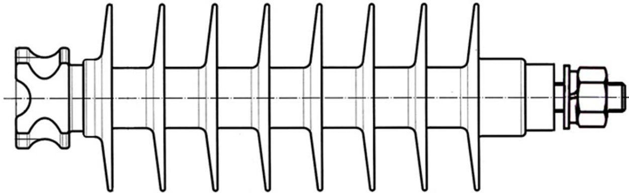
Fig. 33KV 10KN Composite Line Post Insulator
