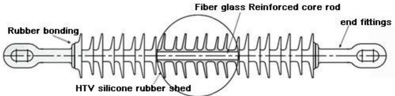
Fig. 69KV 70KN Composite Suspension Insulator
